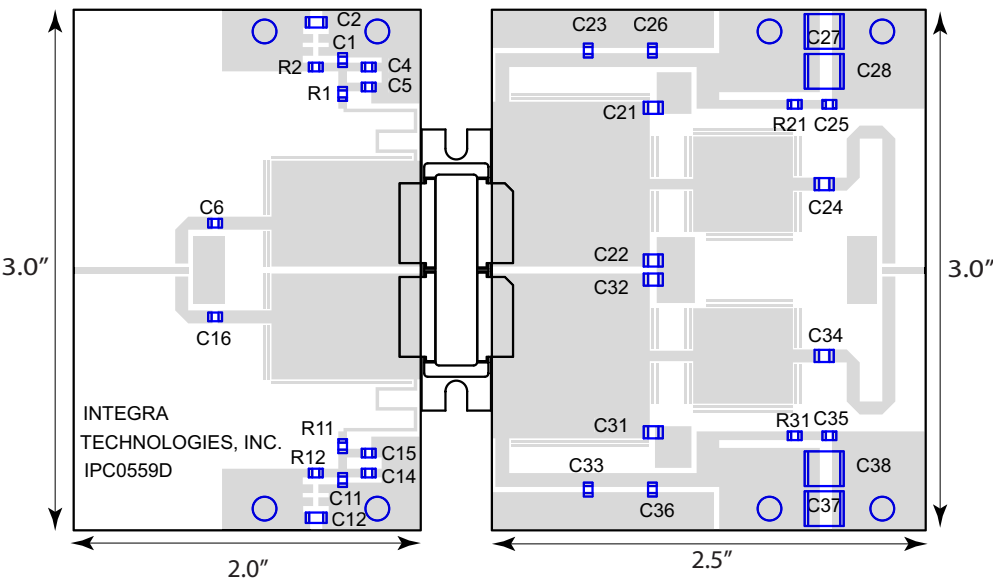
Bill of Materials for IGN1011S3600 Test Fixture
